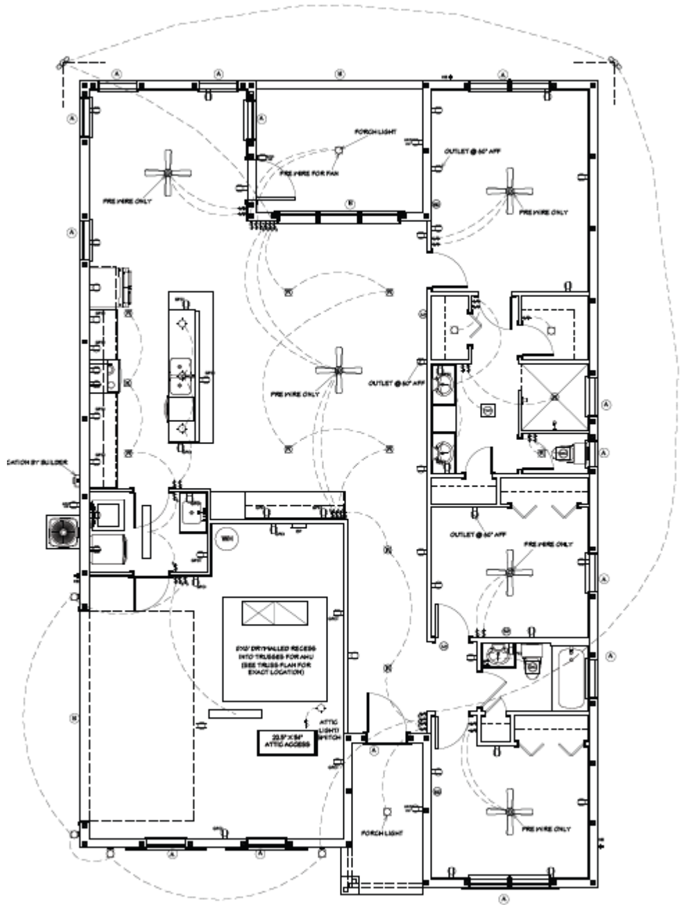
ELECTRICAL PLAN 1/4 IN = 1 FT
