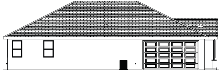
LEFT ELEVATION 1/4 IN = 1 FT
