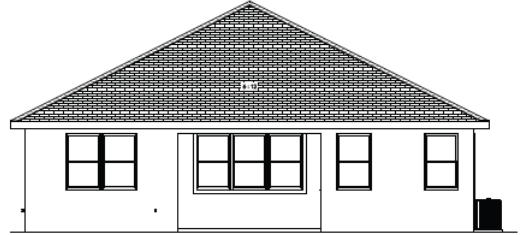
REAR ELEVATION 1/4 IN = 1 FT
